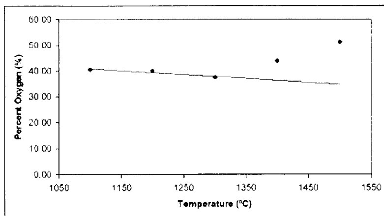
Oxygen Content of BN_xO_y Powders Versus Reactor Temperature from AAVS Reaction of Aqueous H_3BO_3 and NH_3
