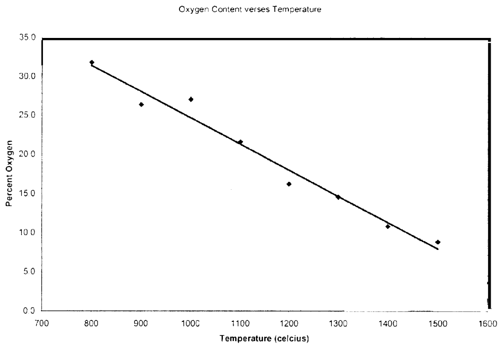
Figure 2. BN_xO_yC_z Powder Oxygen Concentration (% wt.) v.s. AAVS Process Temperature ( N_2 = 1 L/min, NH_3 = 3 L/min) Powder generated from AAVS Reaction between (MeO)_3B and NH_3 .
